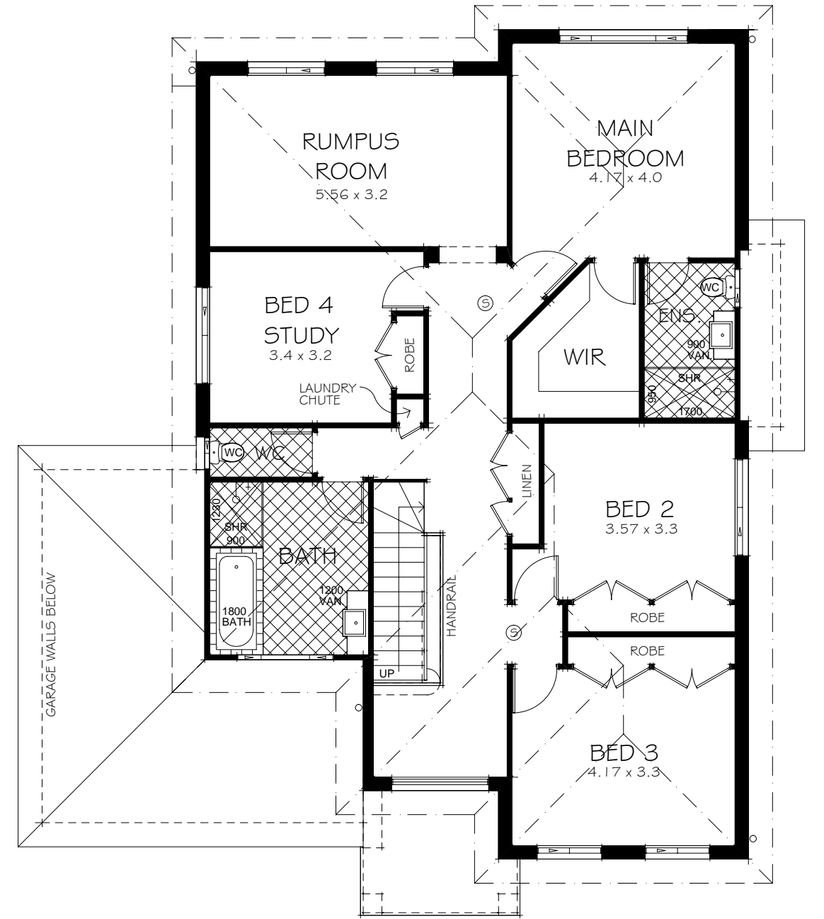
UPPER FLOOR PLAN SCALE 1:100
